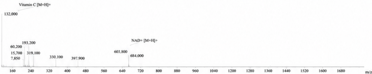
Mass Confirmation
